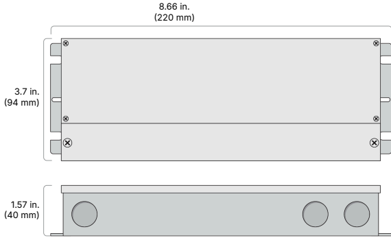
LCI-BNCU-24V96W-J
