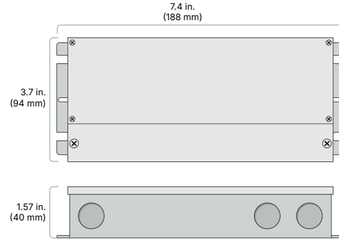
LCI-BNCU-24V60W-J
