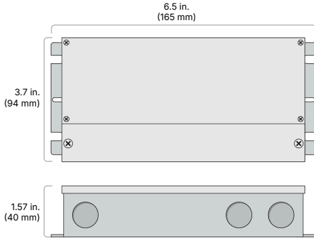
LCI-BNCU-24V30W-J
