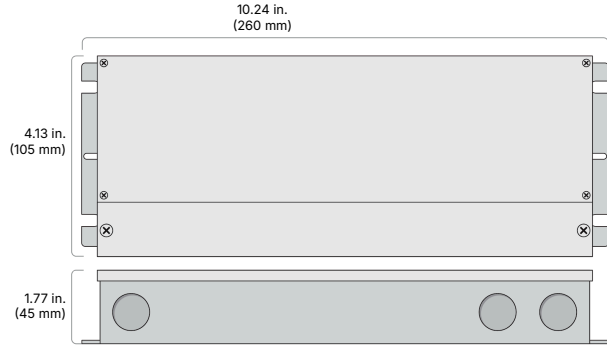
LCI-BNCU-24V200W-J
