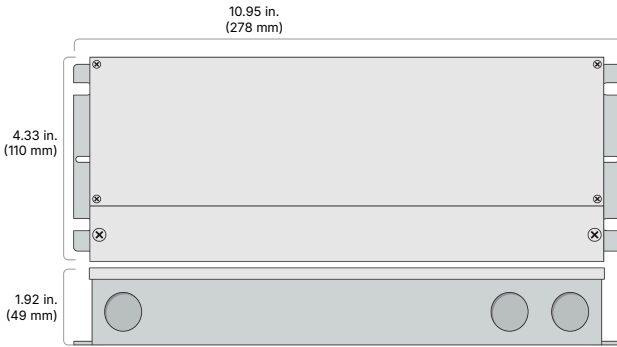
LCI-BNCU-24V300W-J
